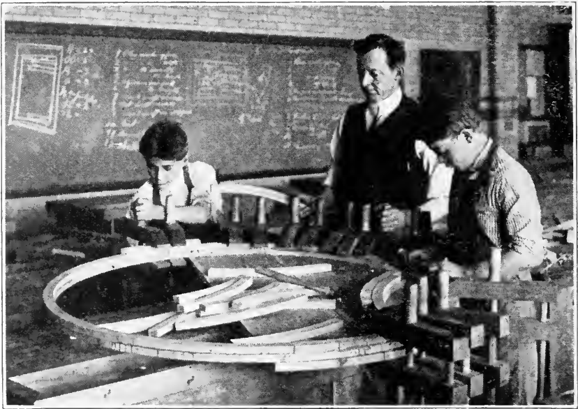
FIG. 406. BUILDING A SEGMENTAL CORE.
